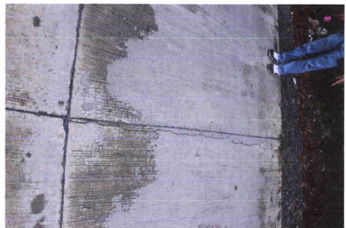
PCCP blocks with transverse cracking acting as weakened plane joints
