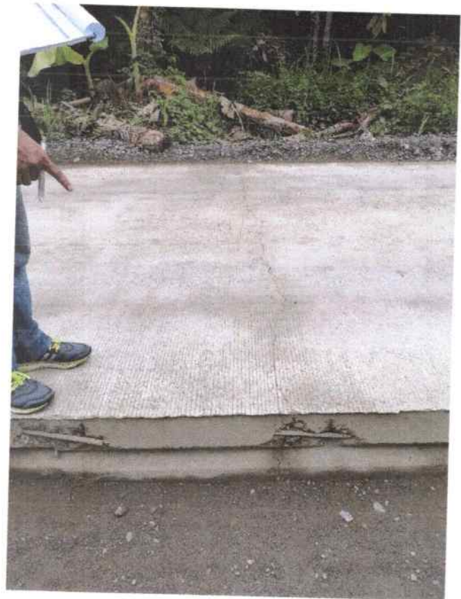
PCCP block with transverse cracking within the middle block
