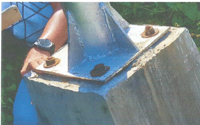
Some base plates are not fitted right with its concrete base/pedestal
